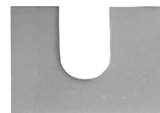
Body Alignment Shim 1/16" Thick, 1/2" Bolt Slot
