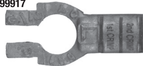
Tru-Crimp® Straight Barrel Battery Terminal 2/0 Ga. Positive
