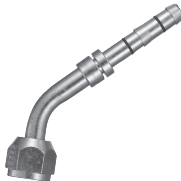
5/16 (-6) x 5/8-18 (-6) 45° Elbow Female O-Ring Short Pilot
