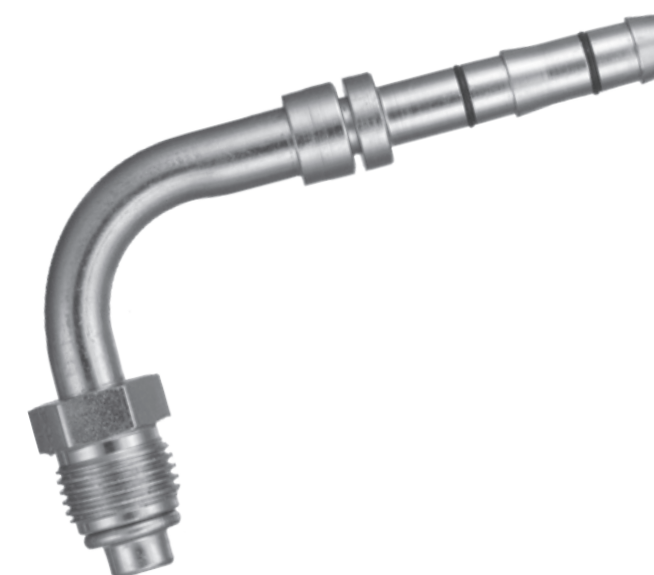
5/16 (-6) x 5/8-18 (-6) 90° Elbow Male O-Ring Short Pilot
