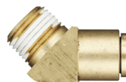
Swivel Male Elbow 45° 1/2 Tube x 3/8 NPT
