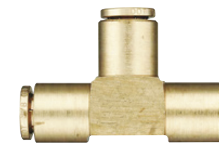
Union Tee 1/2 Tube x 1/2 Tube x 1/2 Tube
