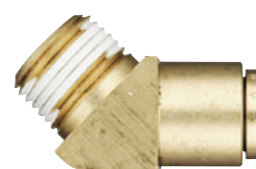
Male Elbow 45° 1/2 Tube x 1/2 NPT
