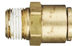
Male Connector 5/8 Tube x 3/8 NPT
