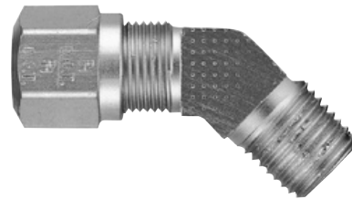
Male Elbow 45° 1/4 Tube x 1/8 NPT
