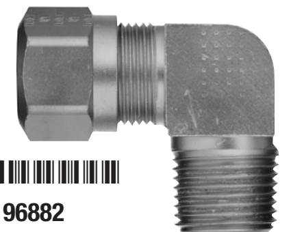
Male Elbow 90° 5/8 Tube x 3/8 NPT
