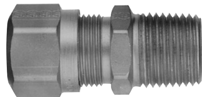
Male Connector 5/8 Tube x 3/8 NPT
