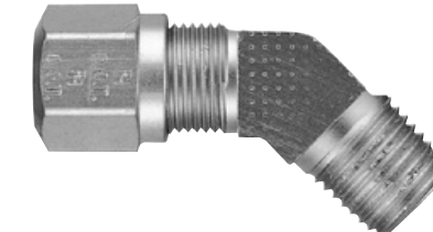
Male Elbow 45° 5/8 Tube x 1/2 NPT
