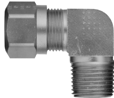
Male Elbow 90° 5/8 Tube x 3/8 NPT
